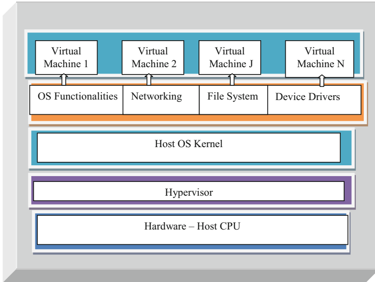
Fig. 22.2 Type-1 hypervisor
